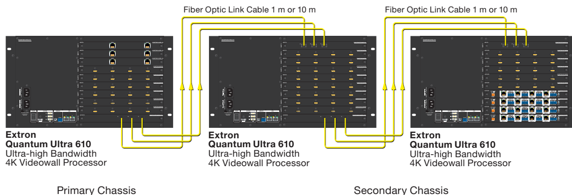
Figure 4. Expansion Card Connection
