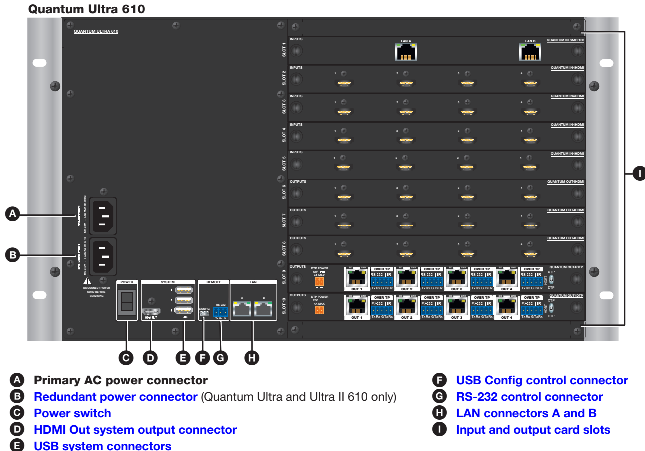
Figure 1. Quantum Ultra 610 Rear Panel
